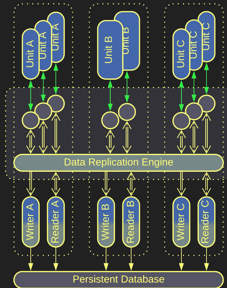
Data Grid
