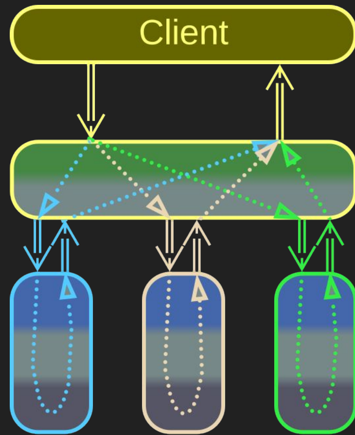
API Composer
