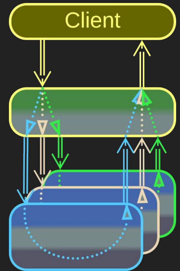
Scatter/Gather, MapReduce
