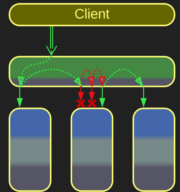
Eventually Consistent Saga
