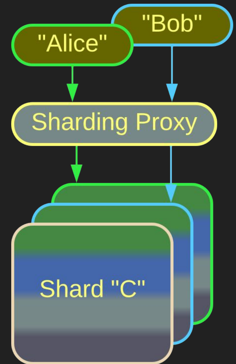
Sharding Proxy
