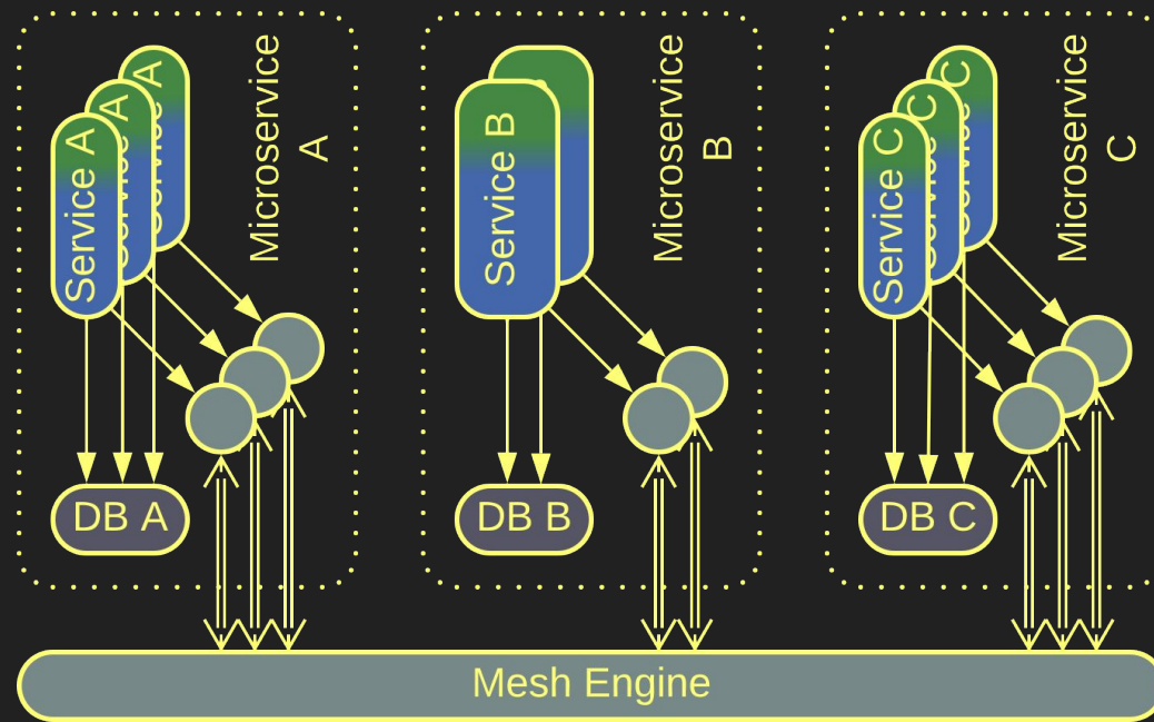
Service Mesh
