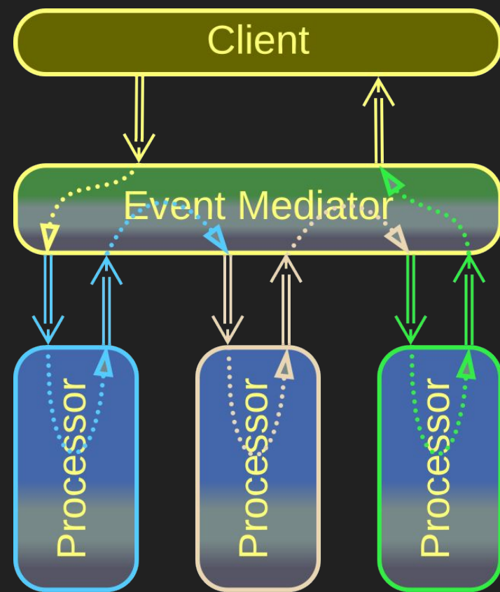
Event Mediator
