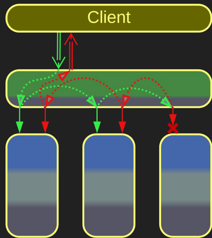
Atomically Consistent Saga
