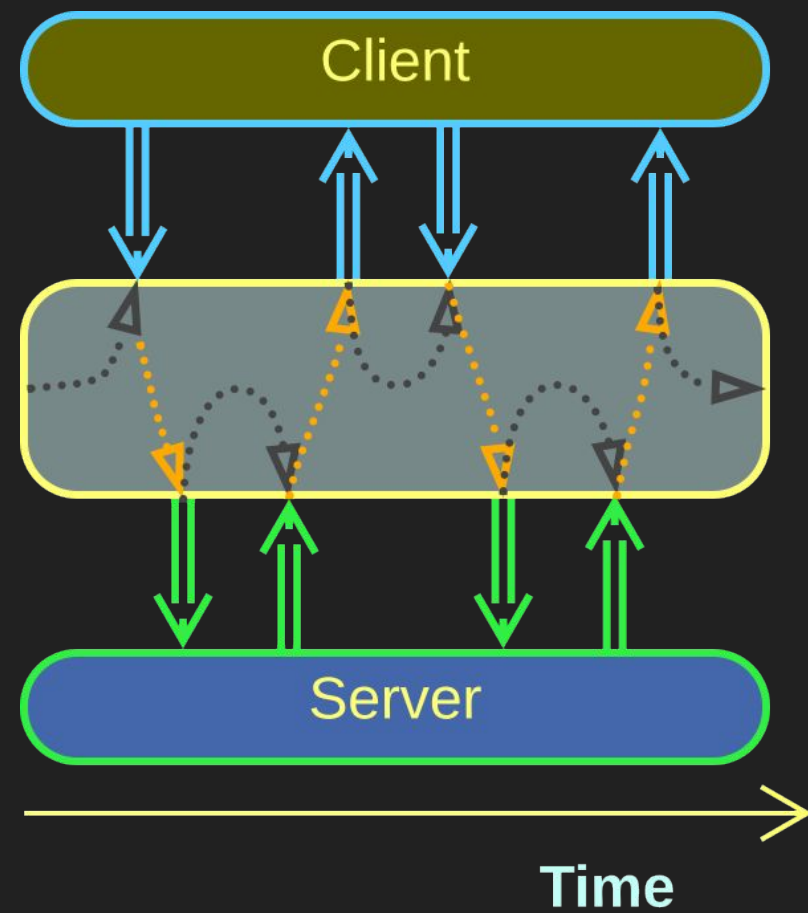
Full Proxy
