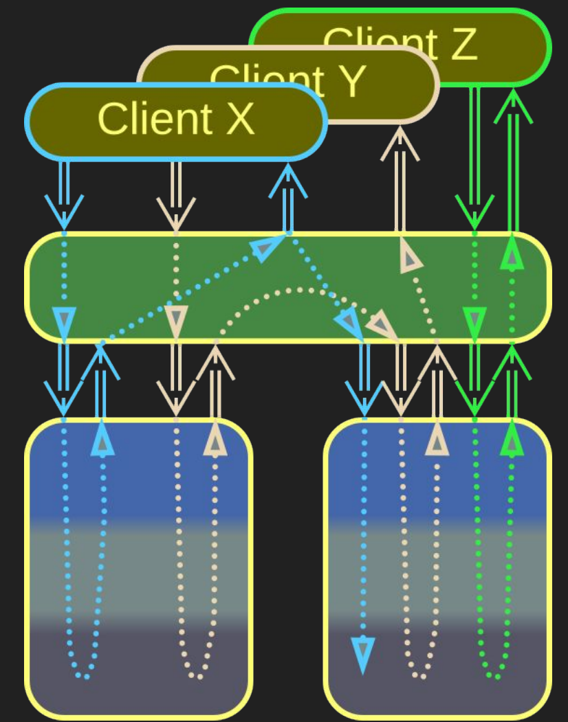
Closed Orchestrator
