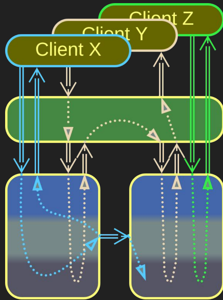
Open Orchestrator
