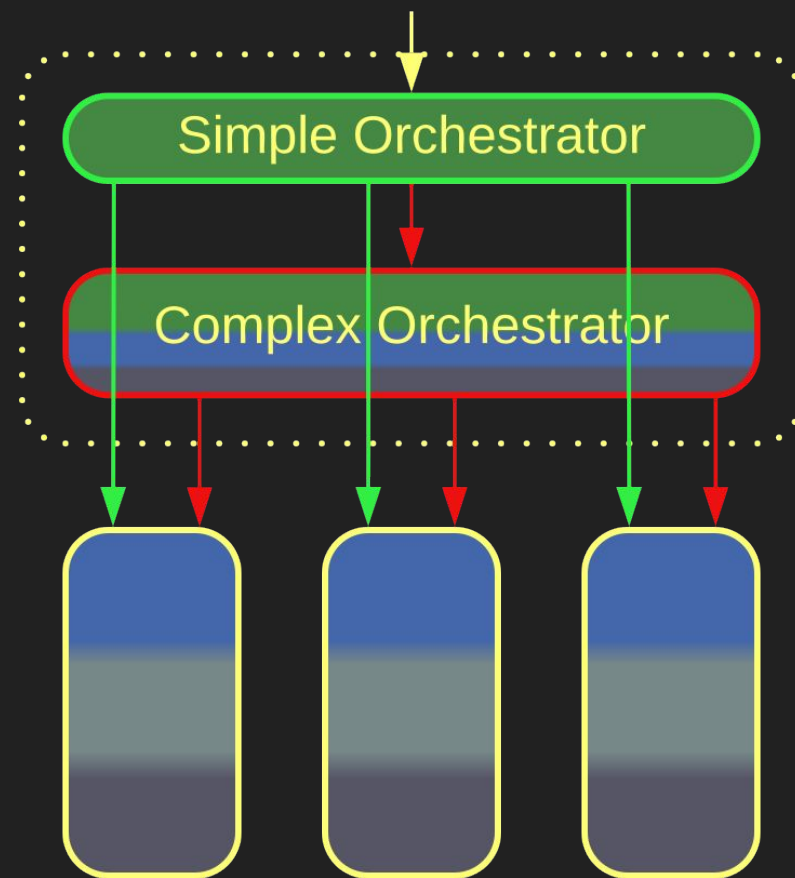
Layered Orchestrator
