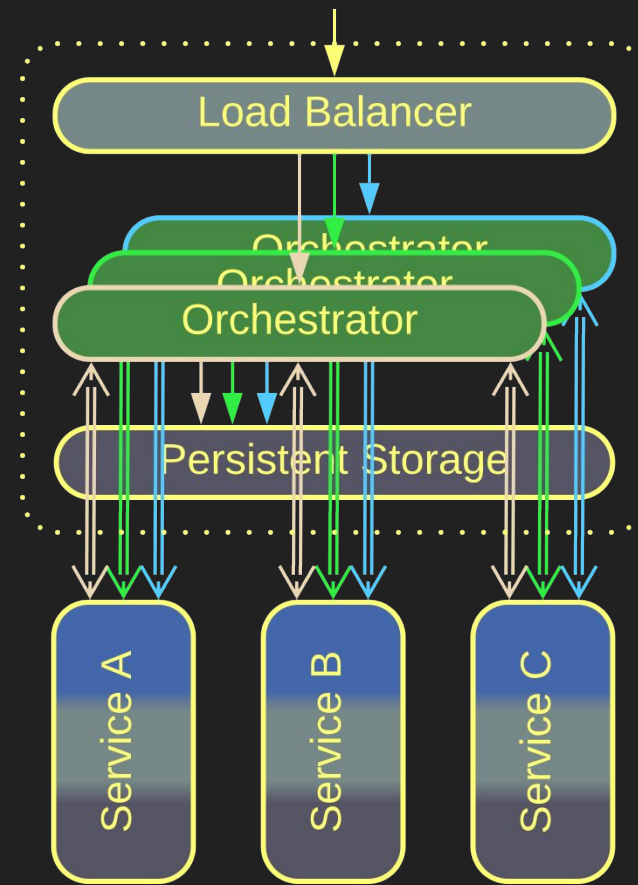
Scaled Orchestrator
